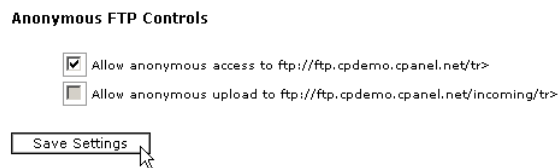
Figure 4.20: Setting Anonymous FTP access
